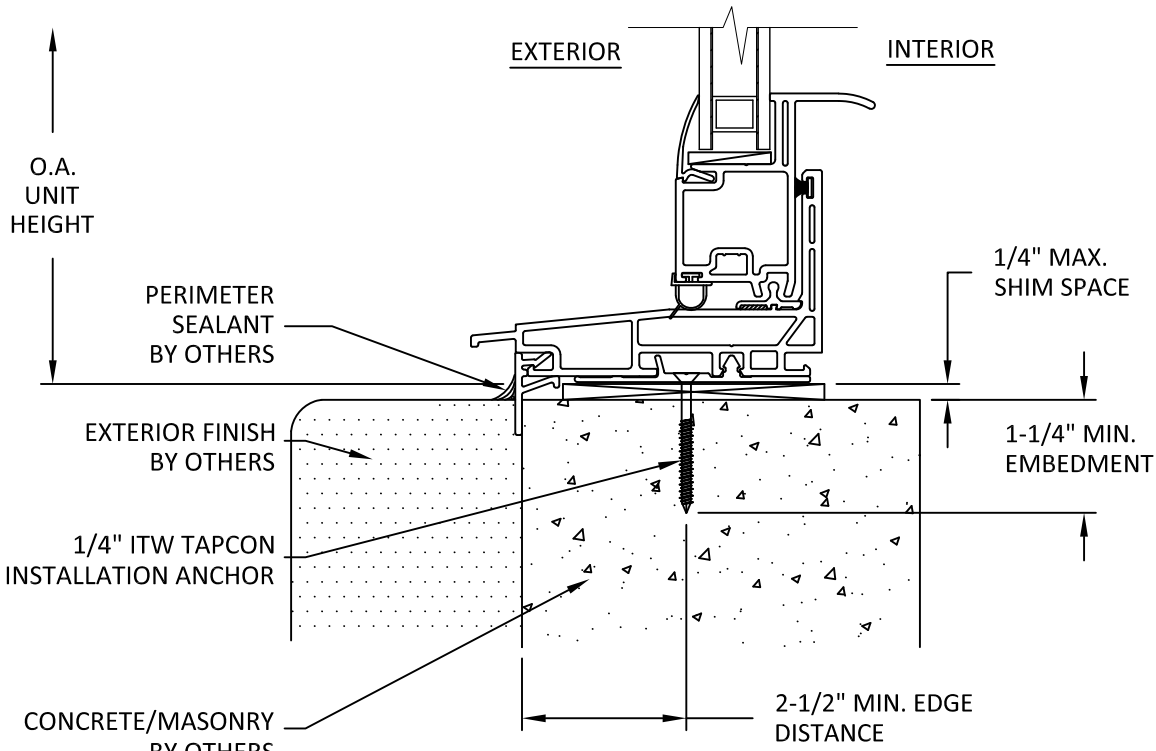
B 3 SILL SECTION THROUGH FRAME INSTALLATION
