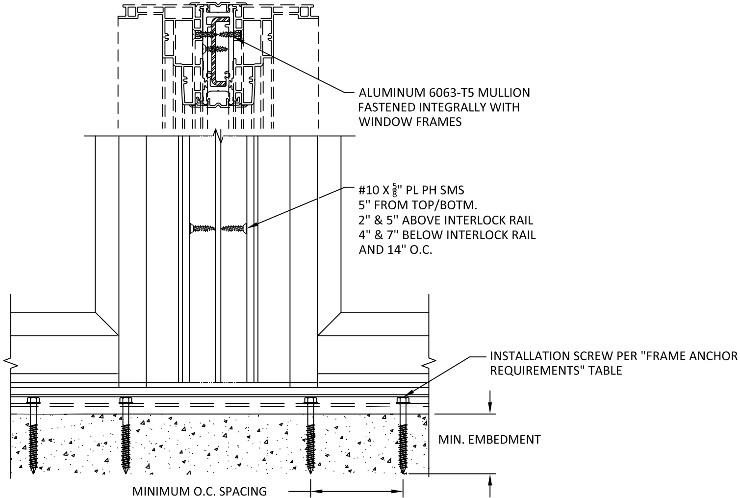
B 2 FRONT VIEW SILL CONDITION UNCLIPPED MULLION (HEAD & JAMB SAME INSTALLATION)
