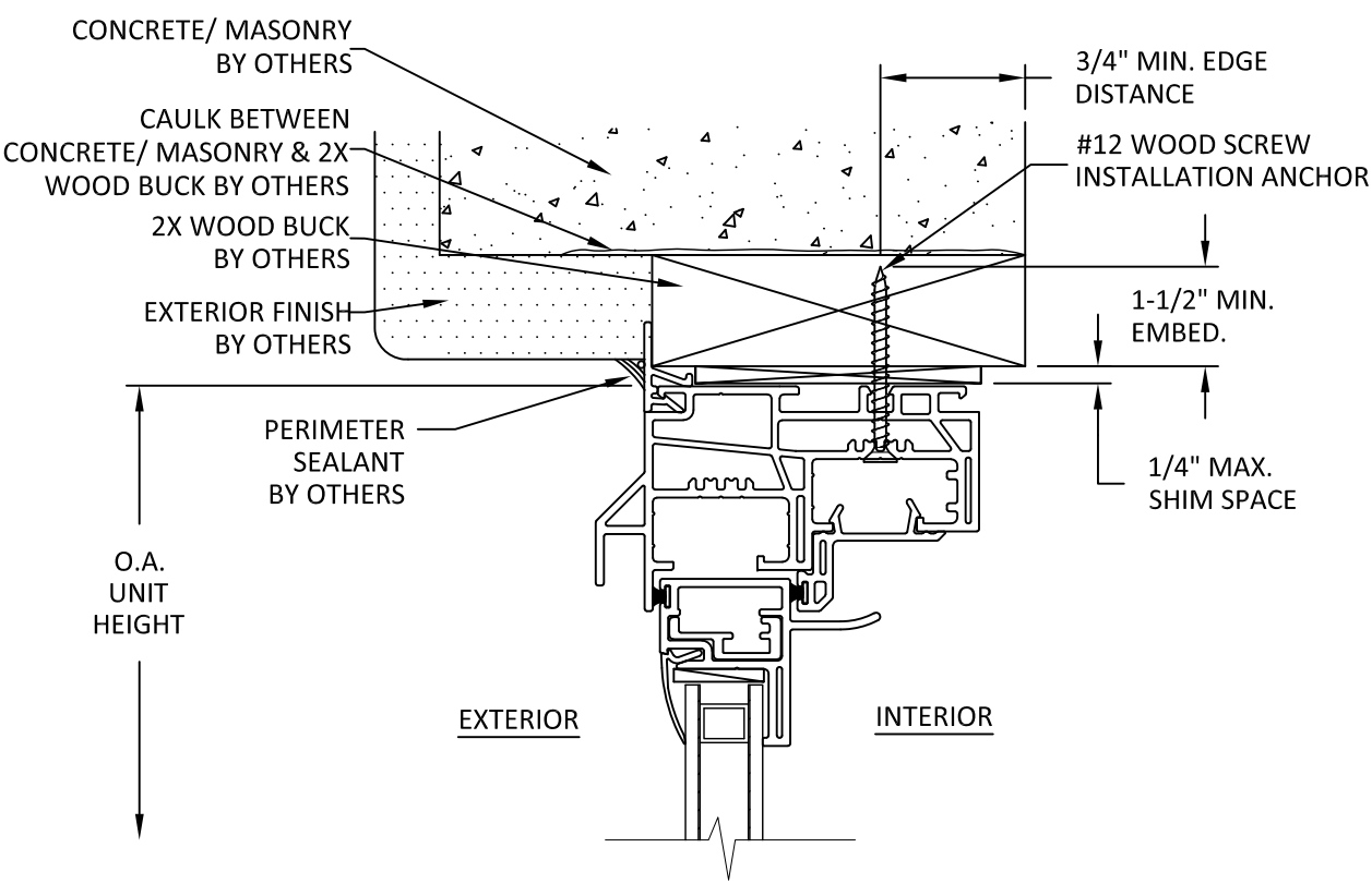
A 3 HEAD SECTION THROUGH FRAME INSTALLATION
