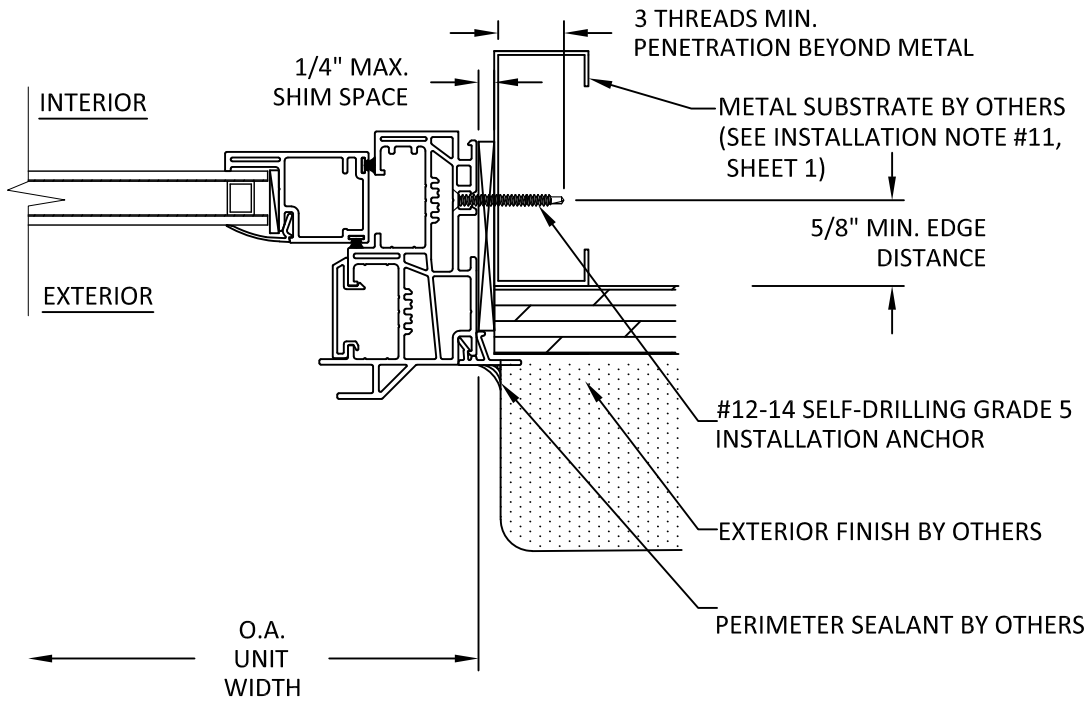
C 3 JAMB SECTION THROUGH FRAME INSTALLATION (HEAD & SILL ARE INSTALLED THE SAME)
