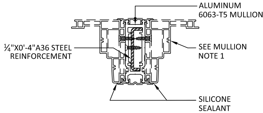
A 2 HORIZONTAL SECTION UNCLIPPED MULLION
